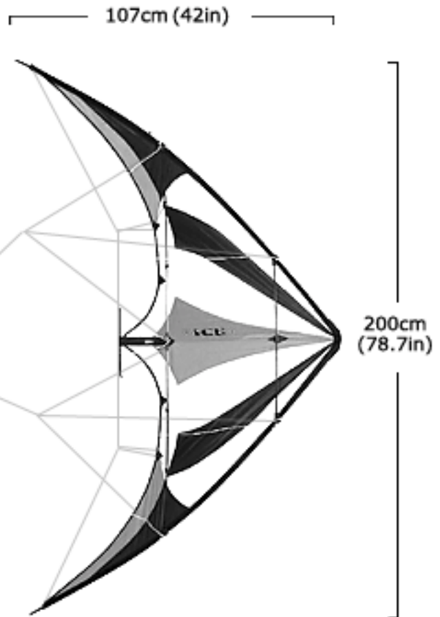
Bottom View
