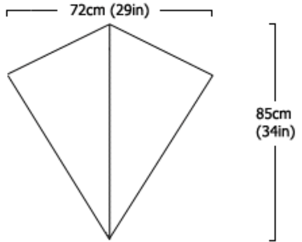
Front view - panels
